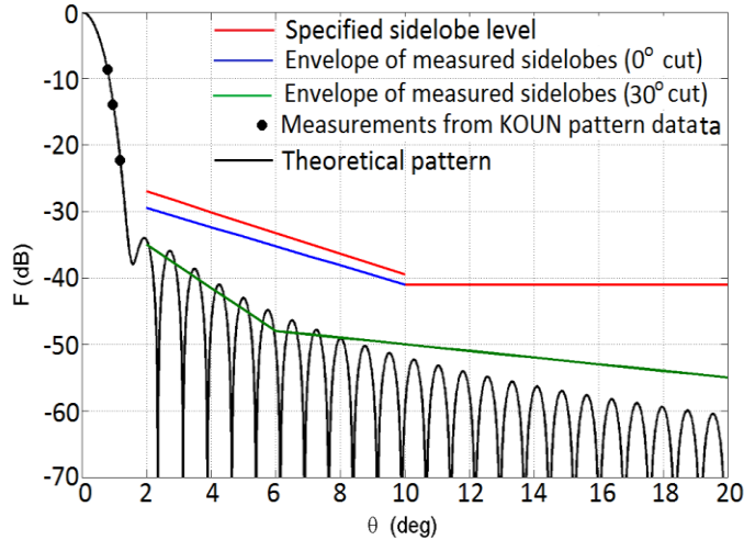
Fig.1. Theoretical one-way power density pattern, 10 \log[ f^2(\theta') ] , as a function of polar angle \theta' for KOUN's antenna (the black line), and comparison with measurements
