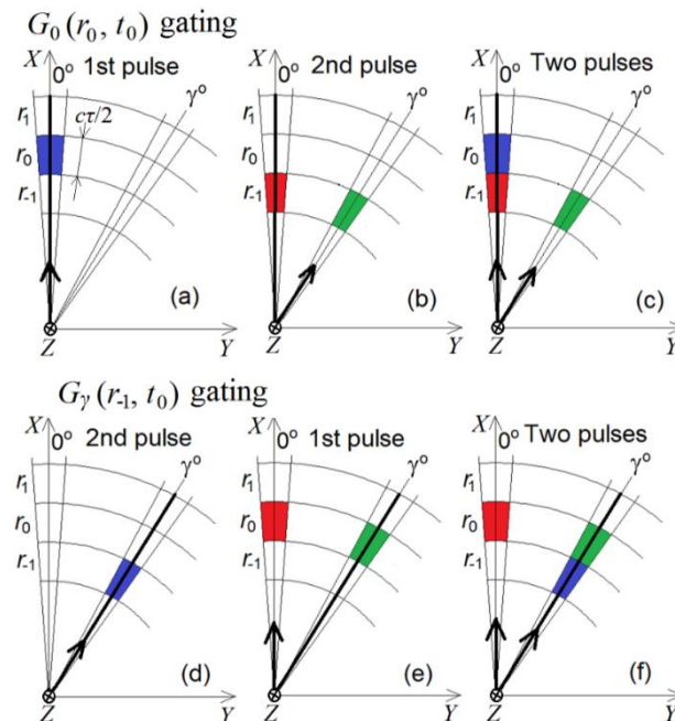
Fig.2. (a - c): Resolution volumes V_6 's (colored sectors) having scatterers that simultaneously and principally contribute to weather echoes sampled with gate G_0(r_0, t_0) . The blue V_6 corresponds to the resolution volume from which echoes are due to m-m coupling, the green and red ones give echoes due to m-s coupling. (d-f): Same as (a-c) but for gate G_\gamma(r_{-1}, t_0) . Transmitting beams are shown with the thick black arrows, and receiving beams are shown with the long thick black lines.
