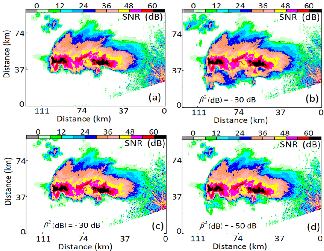
Fig.3. (a): An assumed true SNR (dB) field collected at an elevation angle of 1^\circ with a WSR-88D (i.e., KOUN) on March 31, 2008 at 0334Z. (b): SNR field of the 0^\circ beam showing contamination by m-s coupled power when using dual-beam multiplexing and assuming \beta^2(\text{dB}) = -30 . (c): Retrieved SNR field using 2-term procedure (6)-(7) for \beta^2(\text{dB}) = -30 . (d): As in (b) but for \beta^2(\text{dB}) = -50 .
